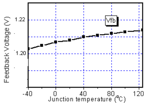
Figure 5. Vfb vs. Temperature
