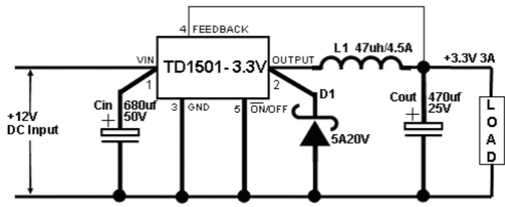
Figure 11. Typical Application of TD1501 For 3.3V
