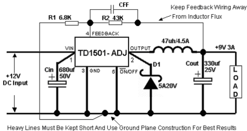
Figure 13. Typical Application of TD1501 For ADJ
